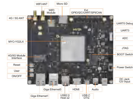
Top View of MYD-YG2LX Development Kit
