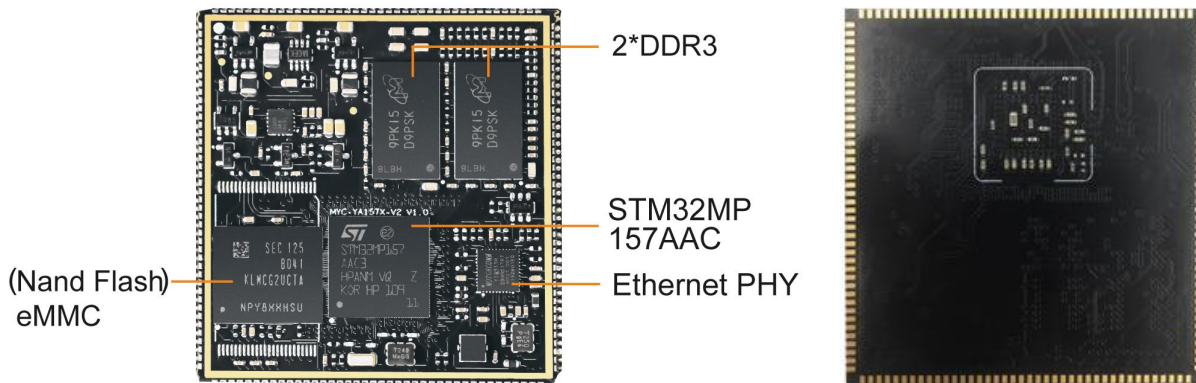
MYC-YA157C-V3 without shielding cover (Top-view and Bottom-view)
