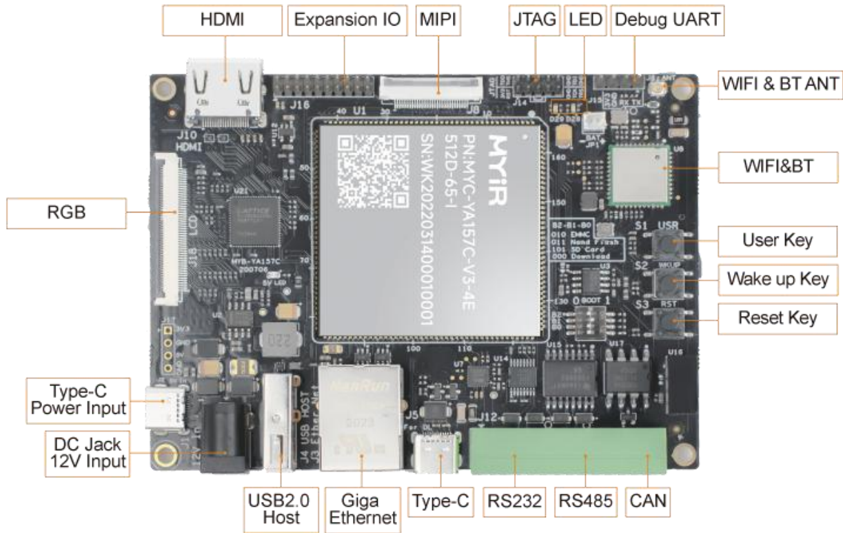
MYD-YA157C-V3 Development Board (Top-view)
