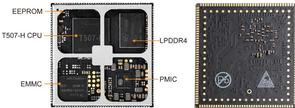
MYC-YT507H Top-view and Bottom-view (delivered with shielding cover installed by default)
