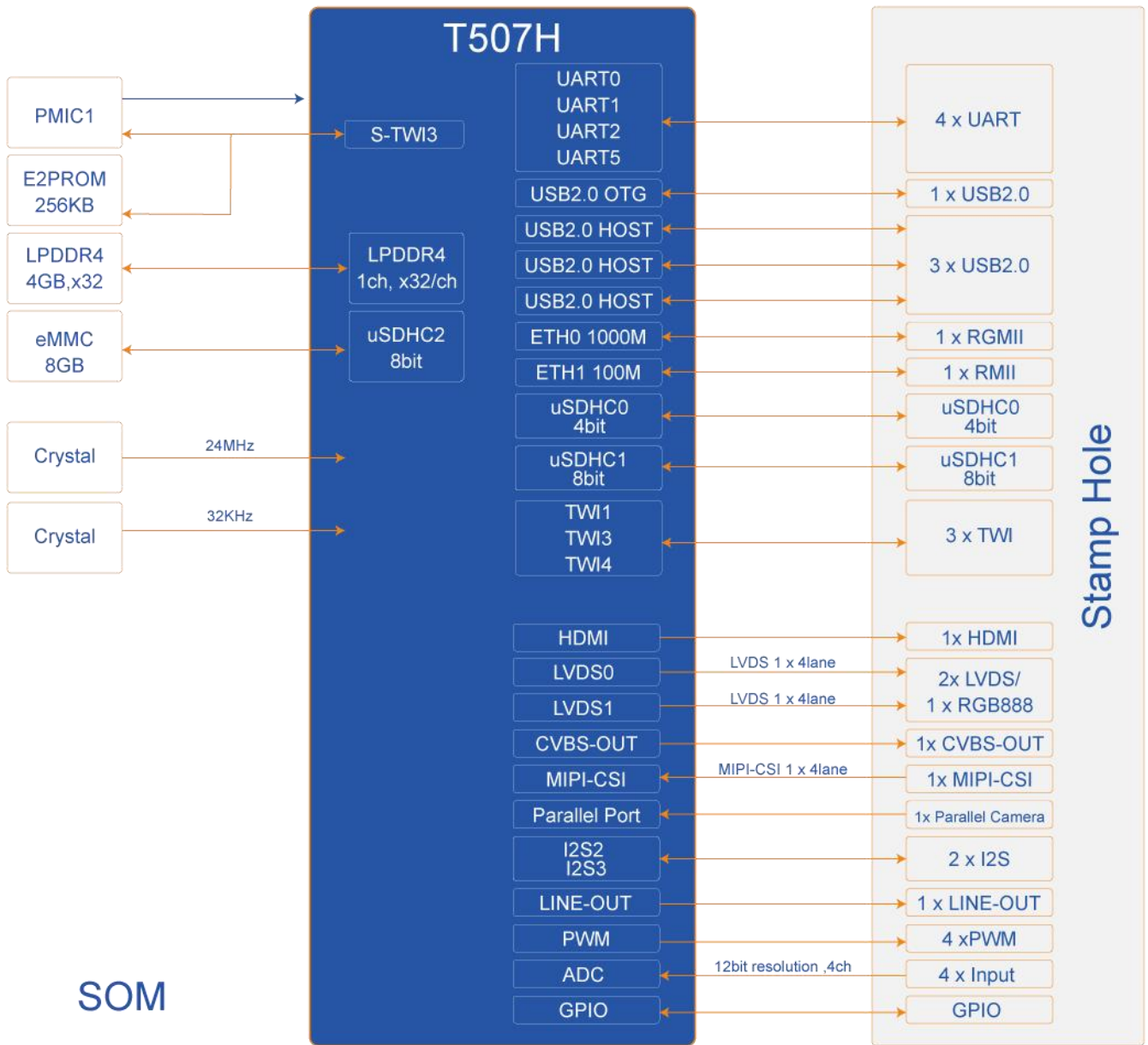
MYC-YT507H Function Block Diagram
