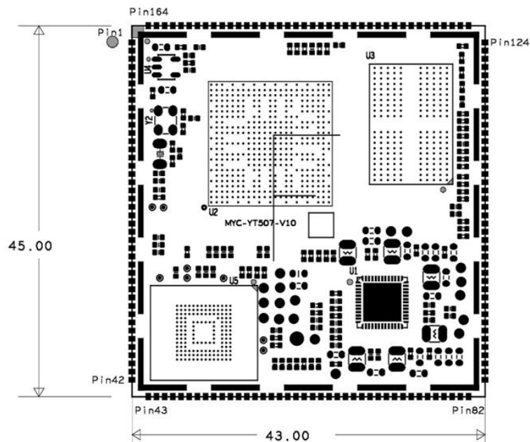
MYC-YT507H Dimensions Chart (Unit: MM)
