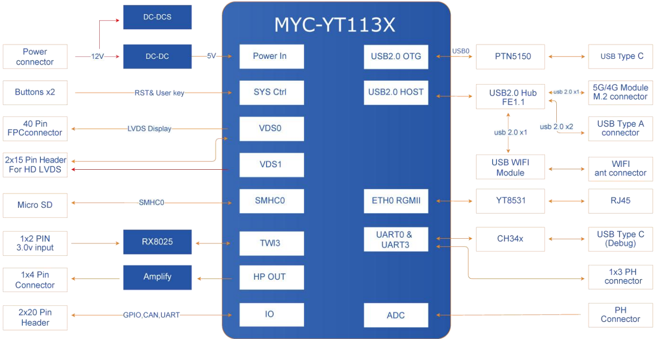
MYD-YT113X Development Board Function Block Diagram
