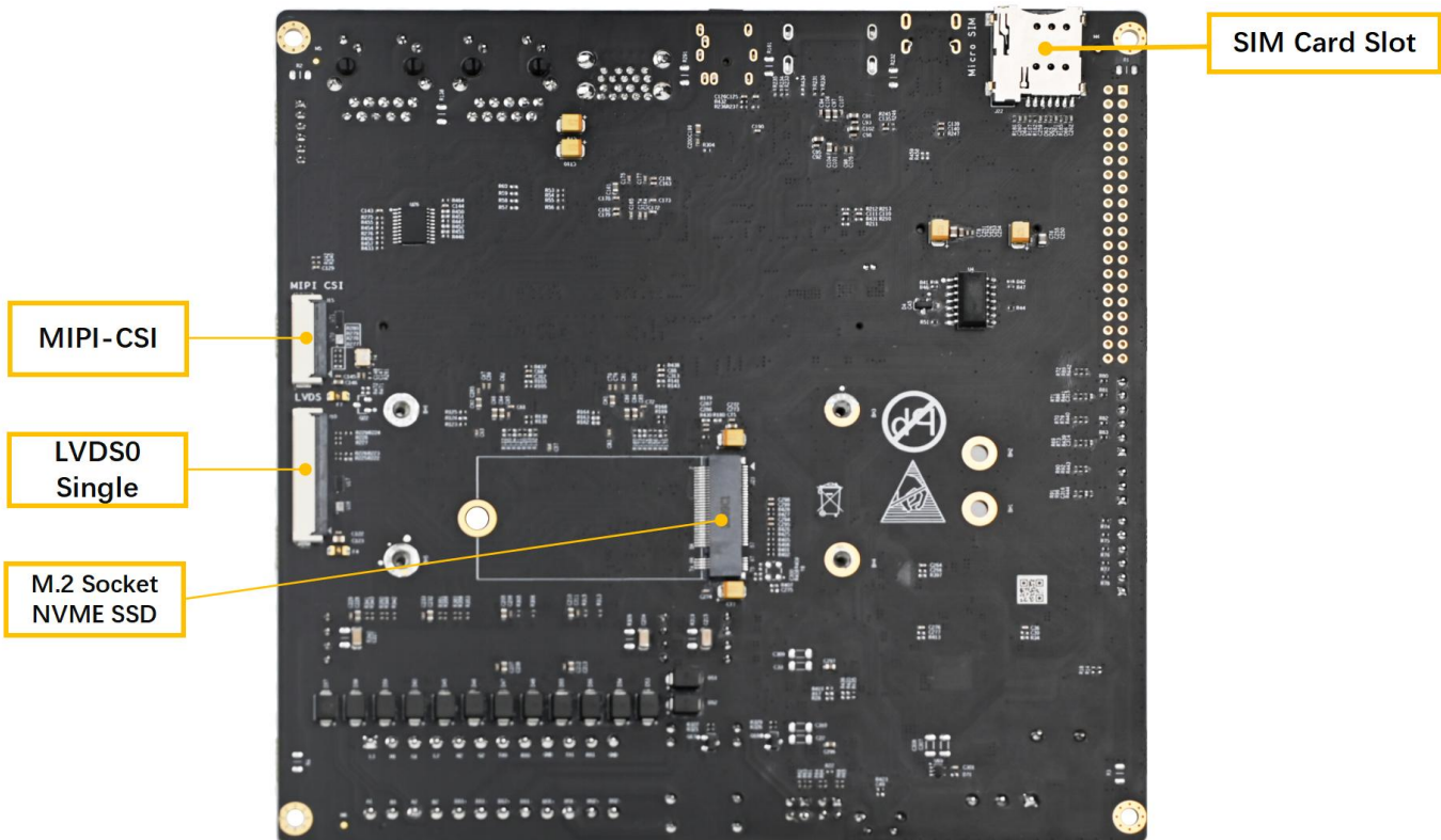
MYD-JD9360 Development Board (Bottom-view)
