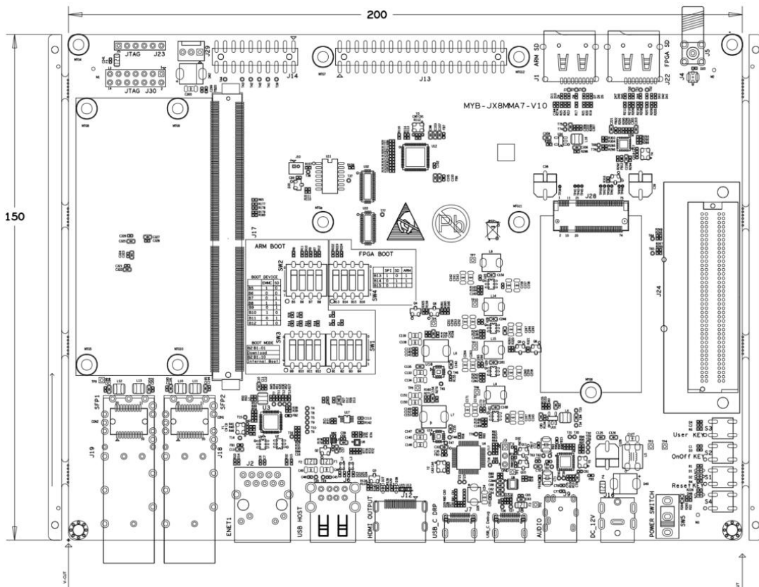
MYD-JX8MMA7 Development Board Dimensions Chart
