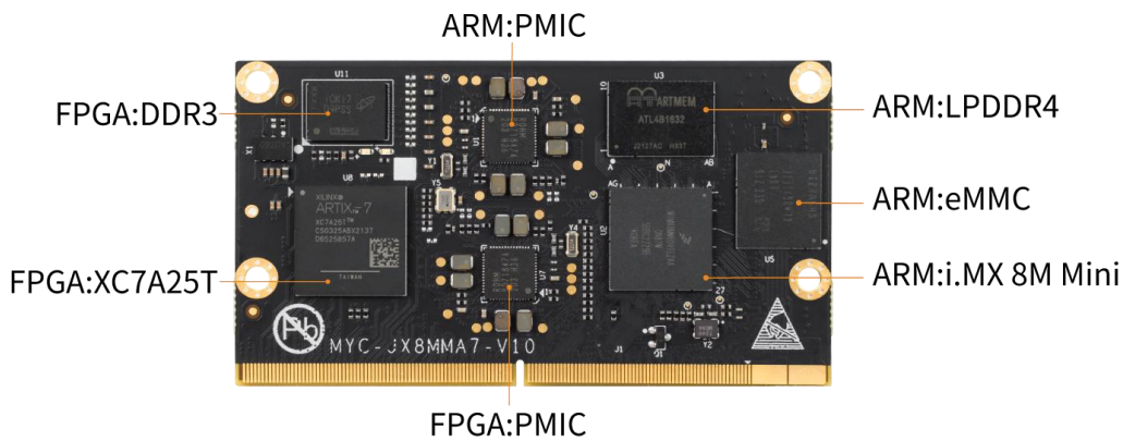
MYC-JX8MMA7 Top-view
