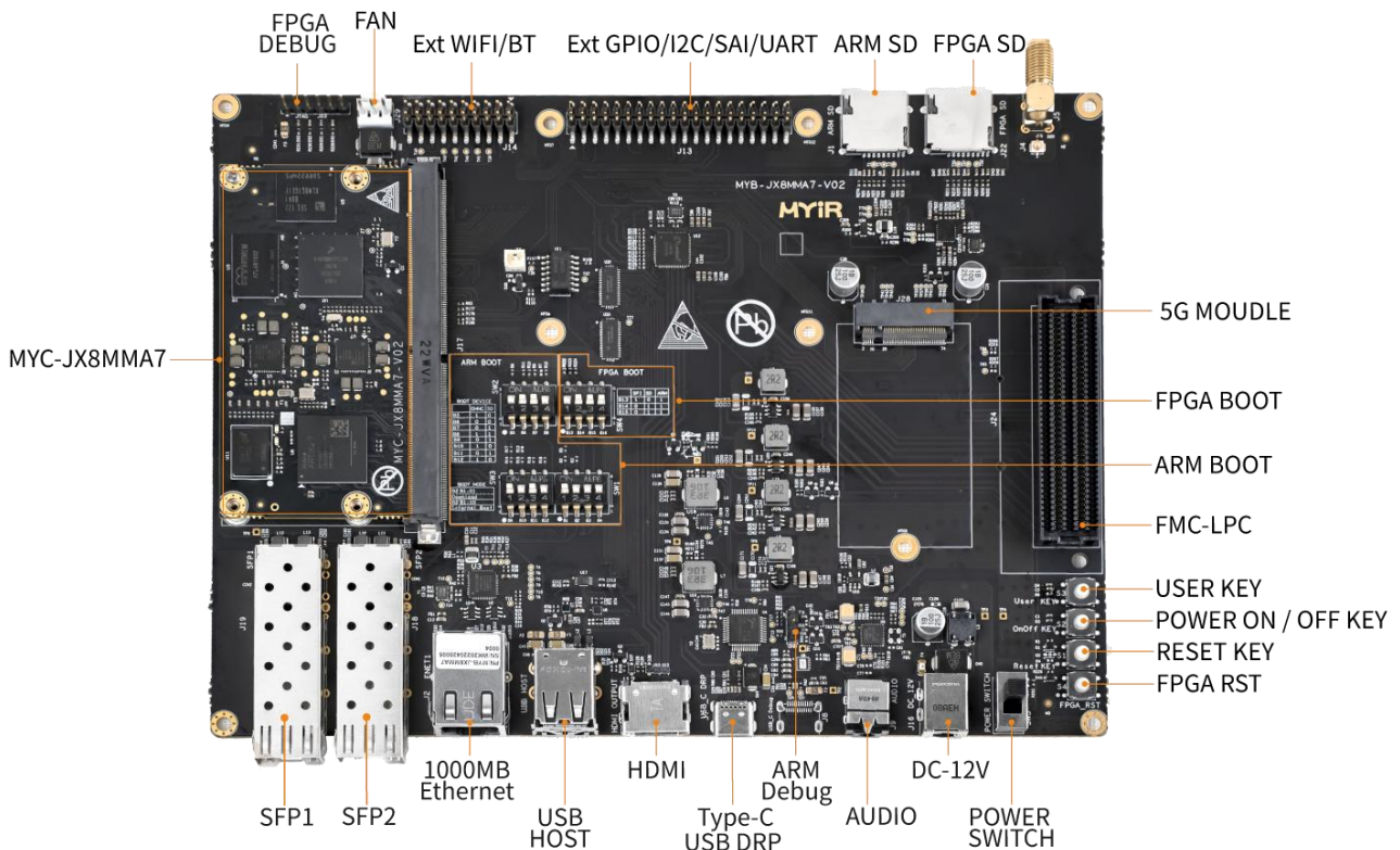
MYD-JX8MMA7 Development Board Top-view
