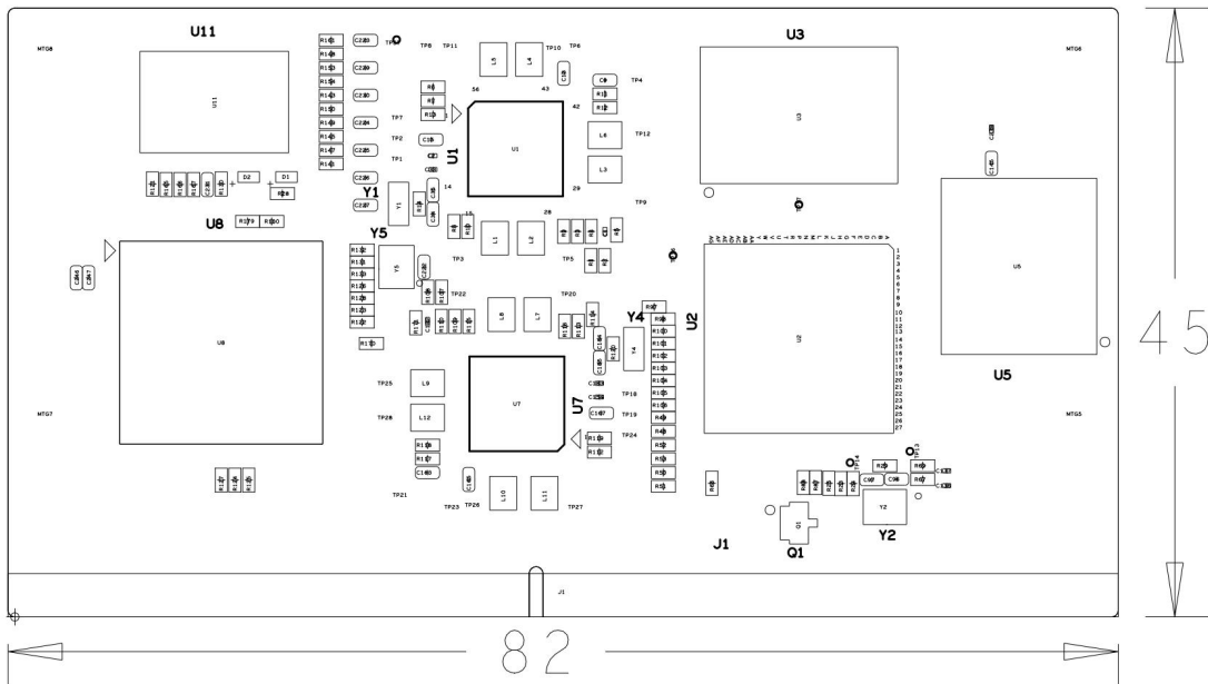
MYC-JX8MMA7 Dimensions Chart
