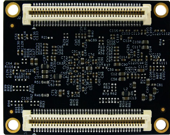
MYC-C335X-GW Bottom-view
