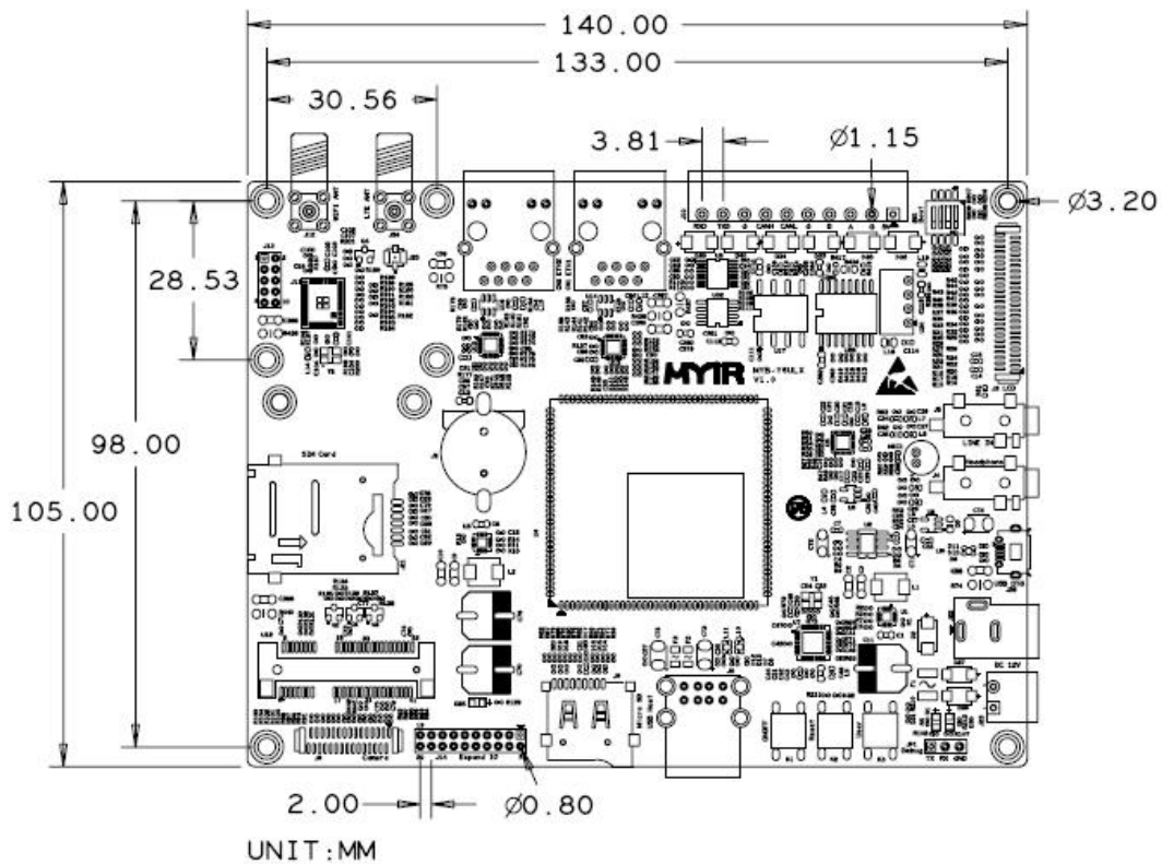
Dimension Chart of MYD-Y6ULX-V2
