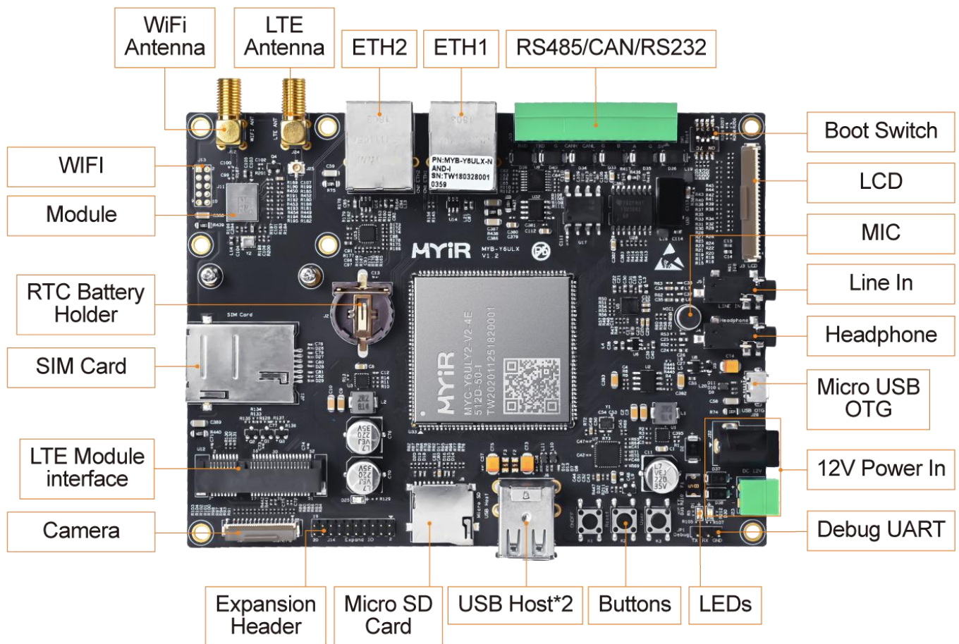
Figure 1-2 MYD-Y6ULX-V2 Development Board Interface Diagram
